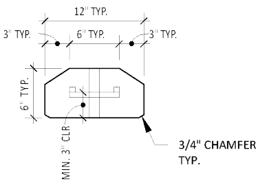
4 SECTION B-B 3/4" = 1'-0"
