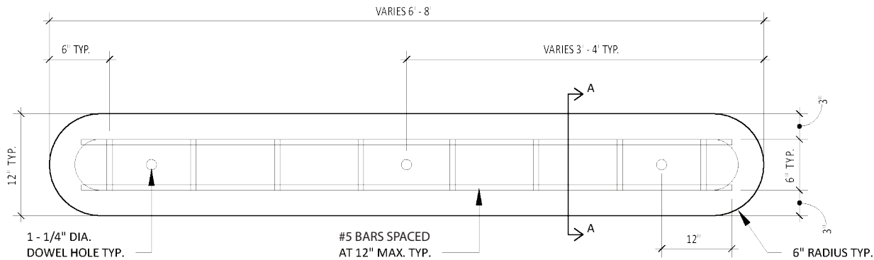
1 PLAN 3/4" = 1'-0"
