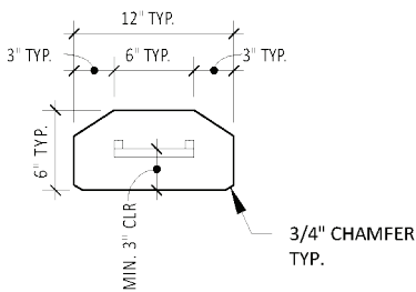
3 SECTION A-A 3/4" = 1'-0"
